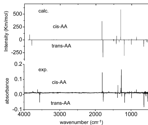
Figure 2. Theoretical and experimental vibrational spectra of cis - and trans -acetic acid. The lower trace is the experimental difference spectrum showing the result of vibrational excitation of the trans conformer in the Ar matrix at 8 K. In the upper trace, the difference spectrum is simulated based on MP2/6-311G++(2d,2p) calculations. The bands of the cis conformer point upward, while the bands due to the trans conformer point downward.
