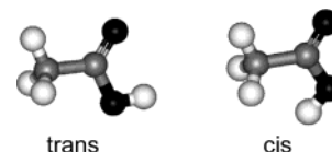
Figure 1. Cis and trans conformers of acetic acid (CH 3 COOH).
